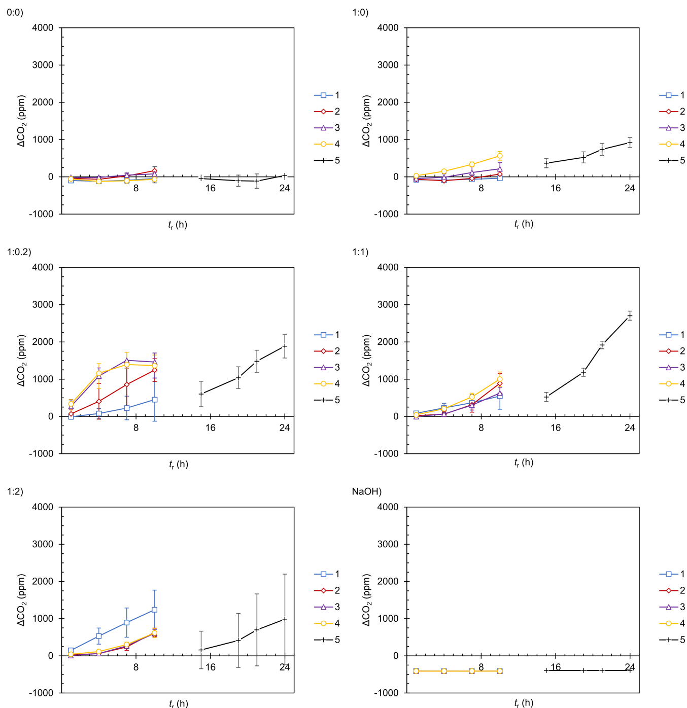
FIGURE 3 Comparison of \text{CO}_2 (ppm) evolution in the vial headspace during MICP over five 24 h turnaround incubation for the treatments with solutions with different urea-to-calcium ratios: distilled water (0:0); urea-to-calcium molar ratio of 1:0; 1:0.2; 1:1; 1:2; and distilled water with adjusted pH of 9.5 with NaOH (NaOH). Incubations after solution additions 1, 2, 3, and 4 were run between 0 and 10 h, and from 14 to 24 h after solution addition 5. A total of four gas measurements were performed during every 10 h incubation period at times t = 1, 3, 7 and 10 h since vial closure. Gas concentrations are the difference between measured average concentrations and atmospheric concentration at t = 0 . Markers and error bars indicate the average and standard deviation of three replicate samples.
